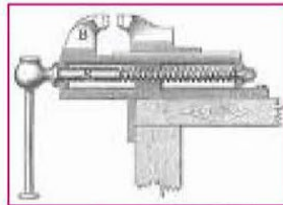
Screw clamping
