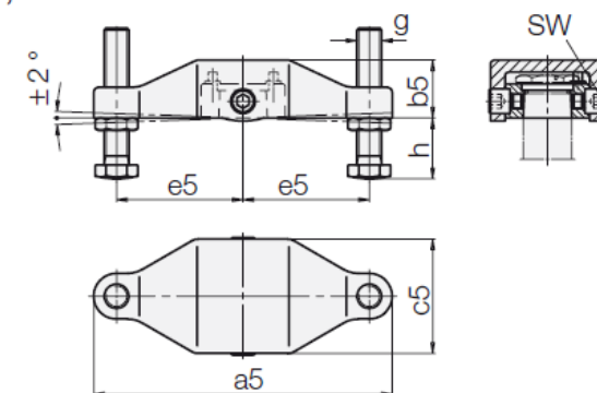
Carrier for double clamping arm 42CrMo4
