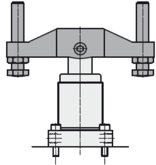
Double clamping arm (500 bar)
