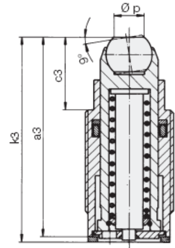
Version with swivel contact bolt
