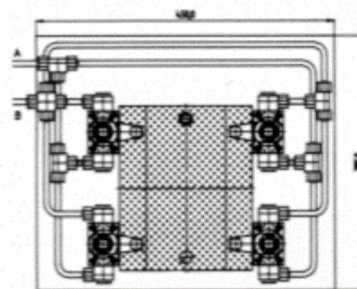
Oil supply through pipes
