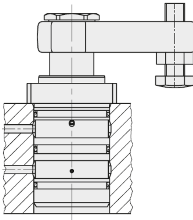
Drilled channels
