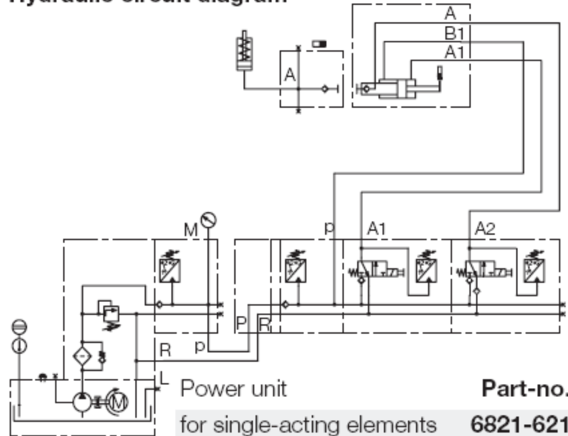
Hydraulic circuit diagram
