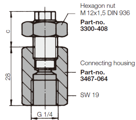
3. Connecting housing and lock nut
