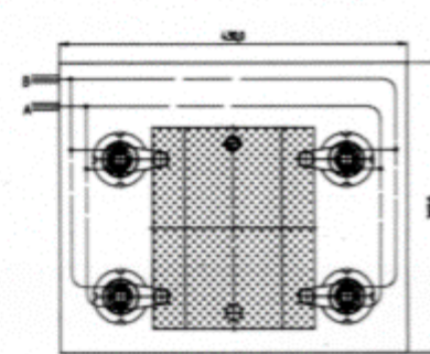
Oil supply through pipes screwed-in swing clamps
