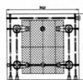
Oil supply through drilled channels manifold-mounted (screw-in) swing clamps
