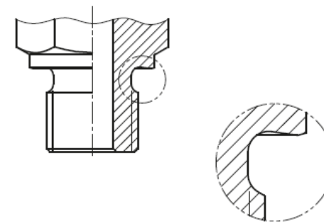
Screwed plug with knife edge
