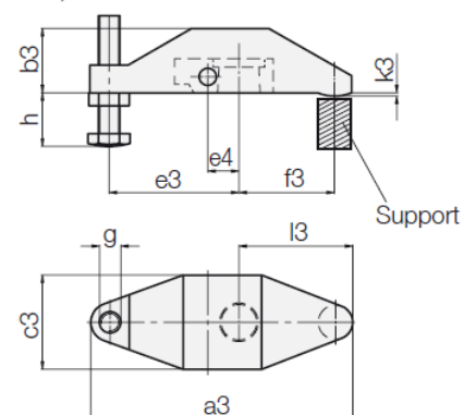
Carrier for clamping arm assembly 42CrMo4
